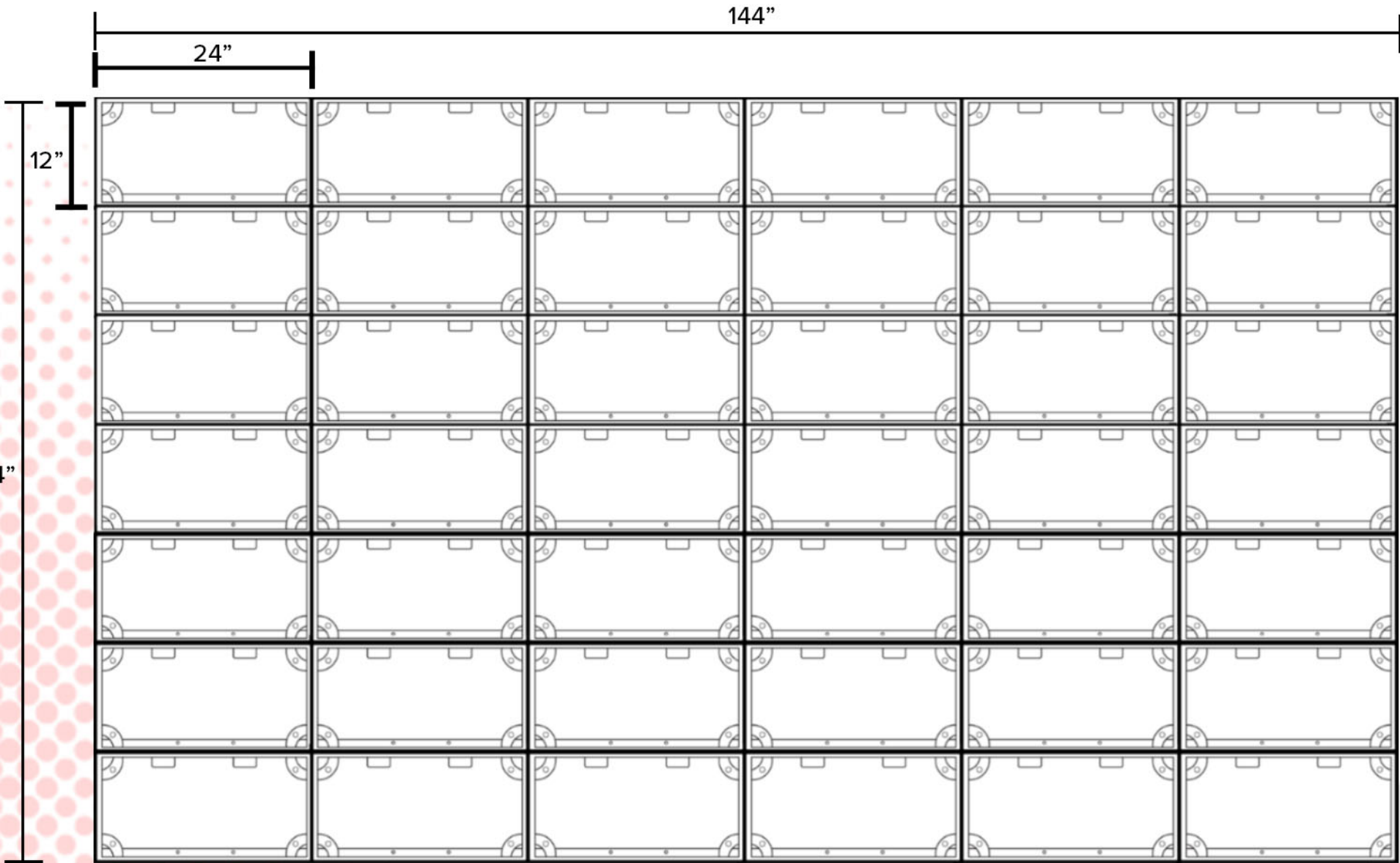
PRIMARY DISPLAY REAR VIEW
